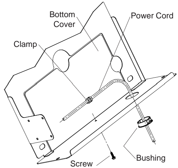
220V POWER CORD DETAIL
